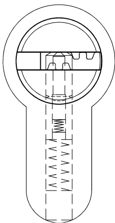
Typical RH cylinder section
